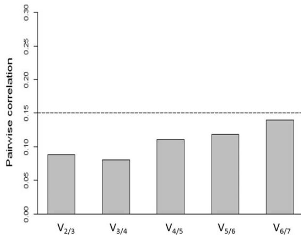
Fig. 3. geNorm pairwise variation (V) analysis to determine optimal number of reference genes for normalization in RT-qPCR reaction. The dotted line corresponds to the cut-off value of 0.15 for accurate normalization.
