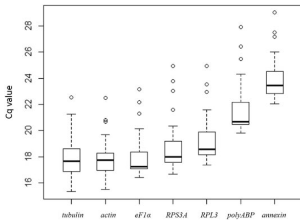
Fig. 2. Distribution of expression levels of candidate reference genes in the 21 wing discs. The expression level is shown through the Cq value.
