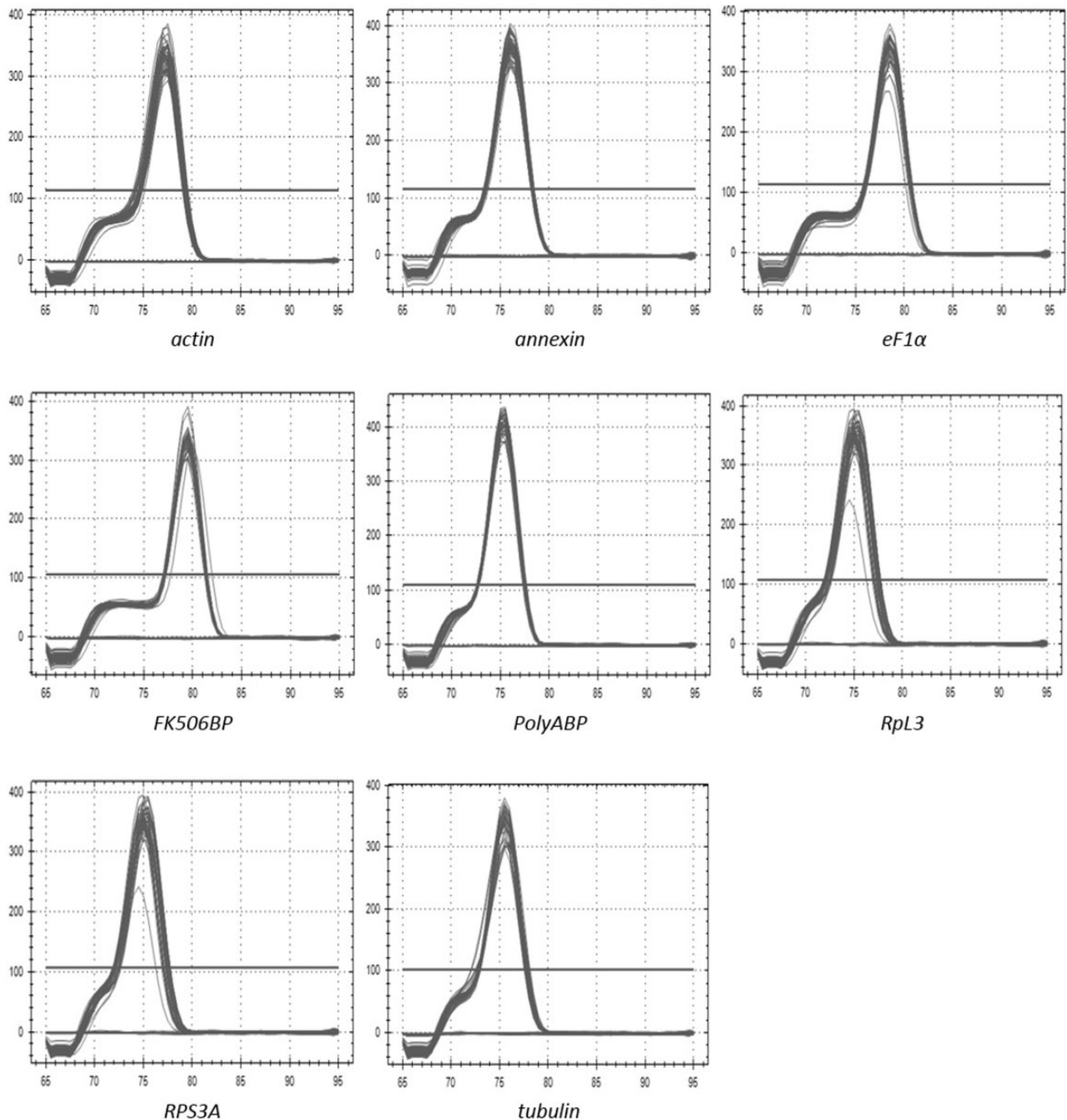
Fig 1. qPCR primer specificity. Melt curves, for all genes, are determined by plotting the negative first derivative of fluorescence versus the temperature in Celsius ( -d(\text{RFU})/dT ).
